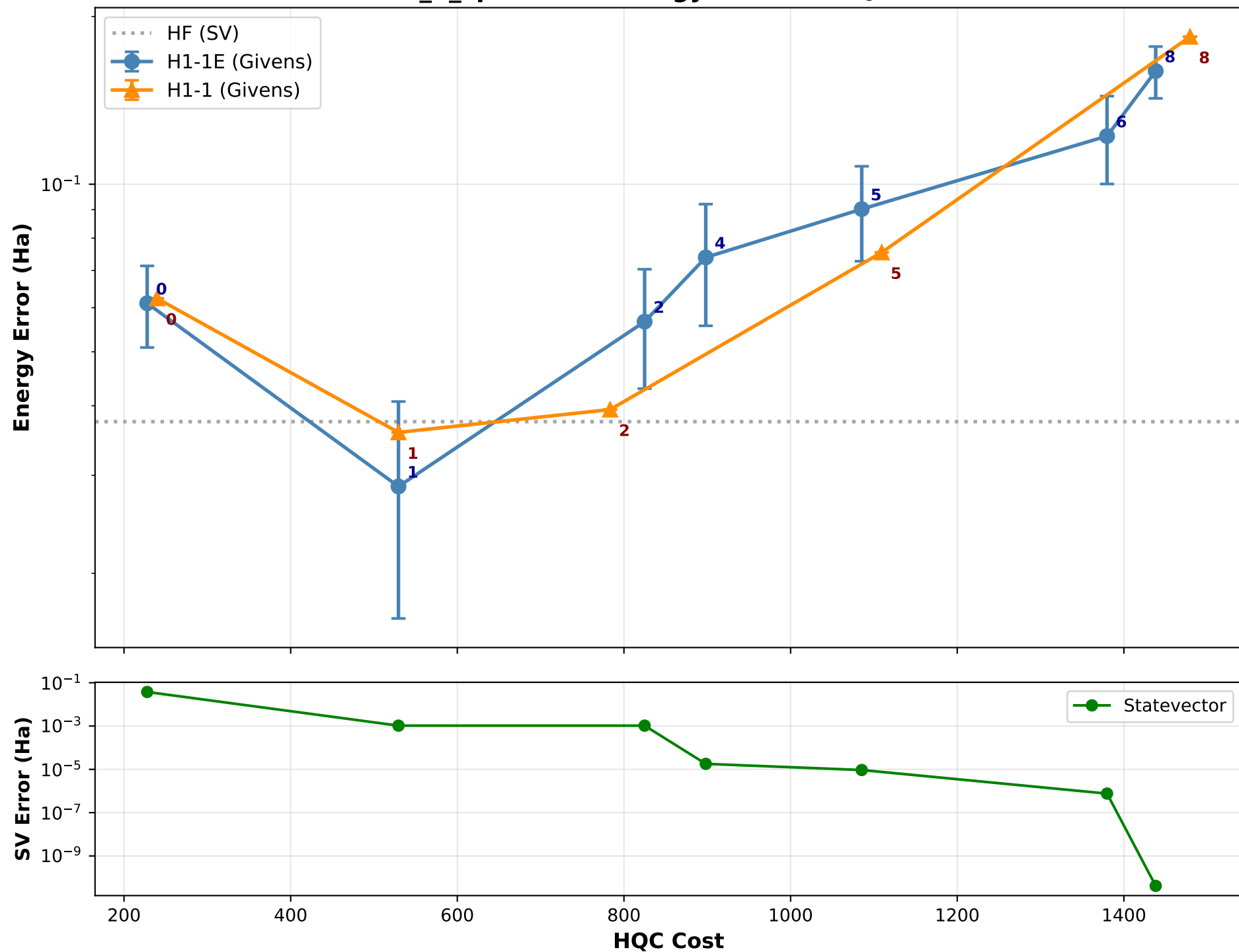
LiH_6_spinorbs - Energy Error vs HQC Cost
