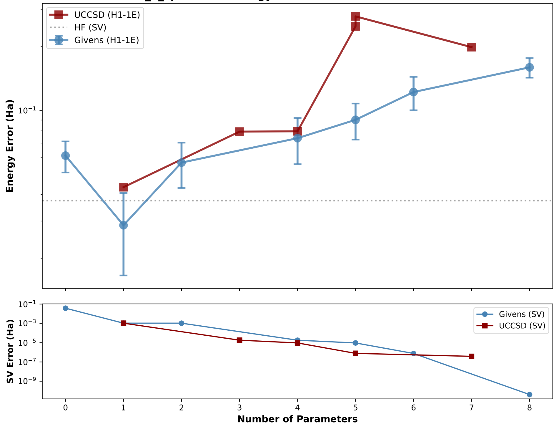
LiH_6_spinorbs - Energy Error vs Number of Parameters
