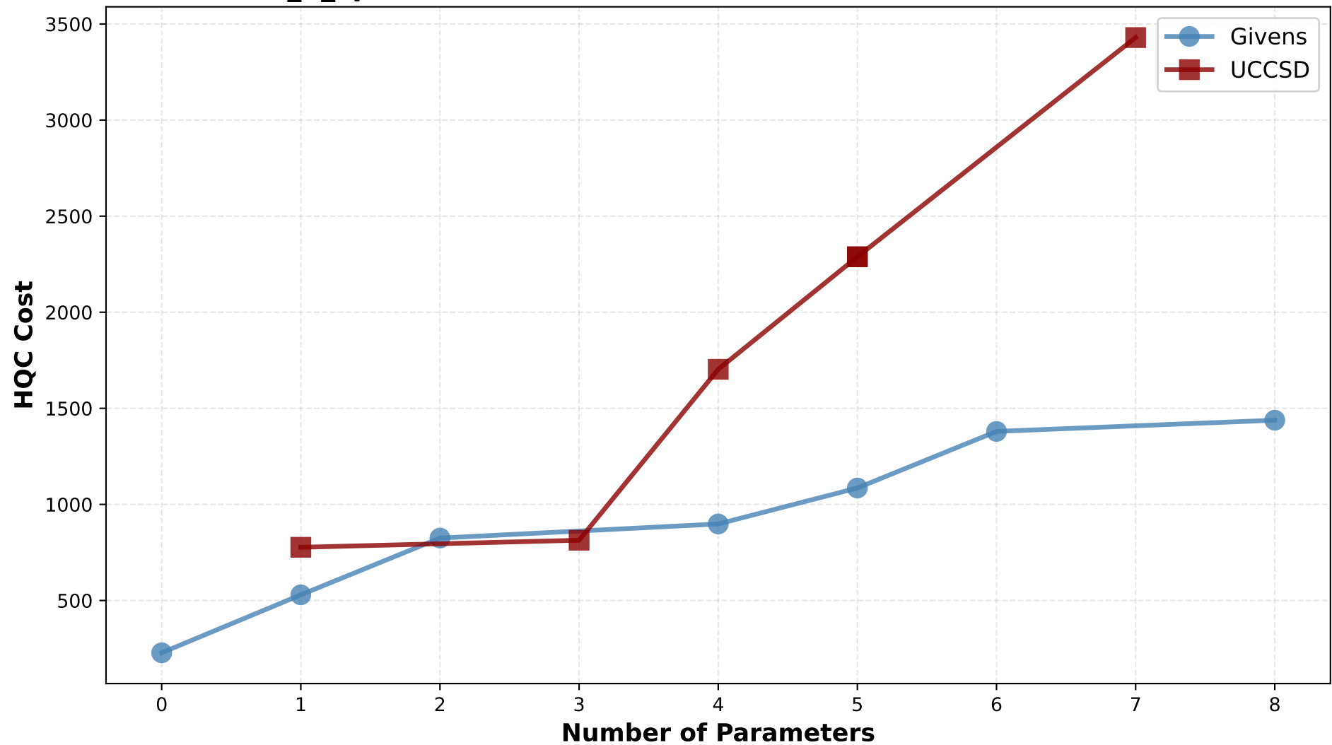
LiH_6_spinorbs - HQC Cost vs Number of Parameters (H1-1E)
