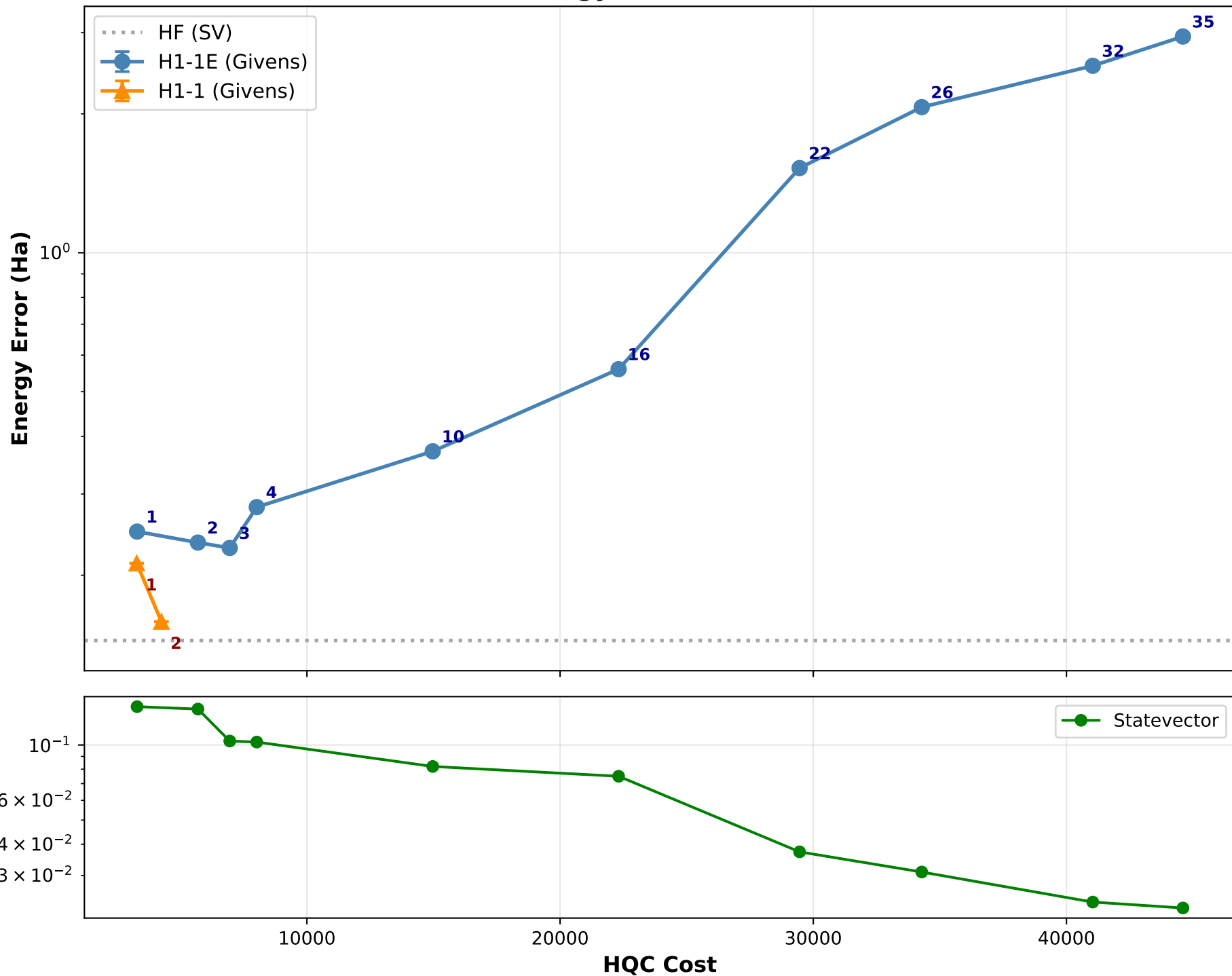
N2 - Energy Error vs HQC Cost
