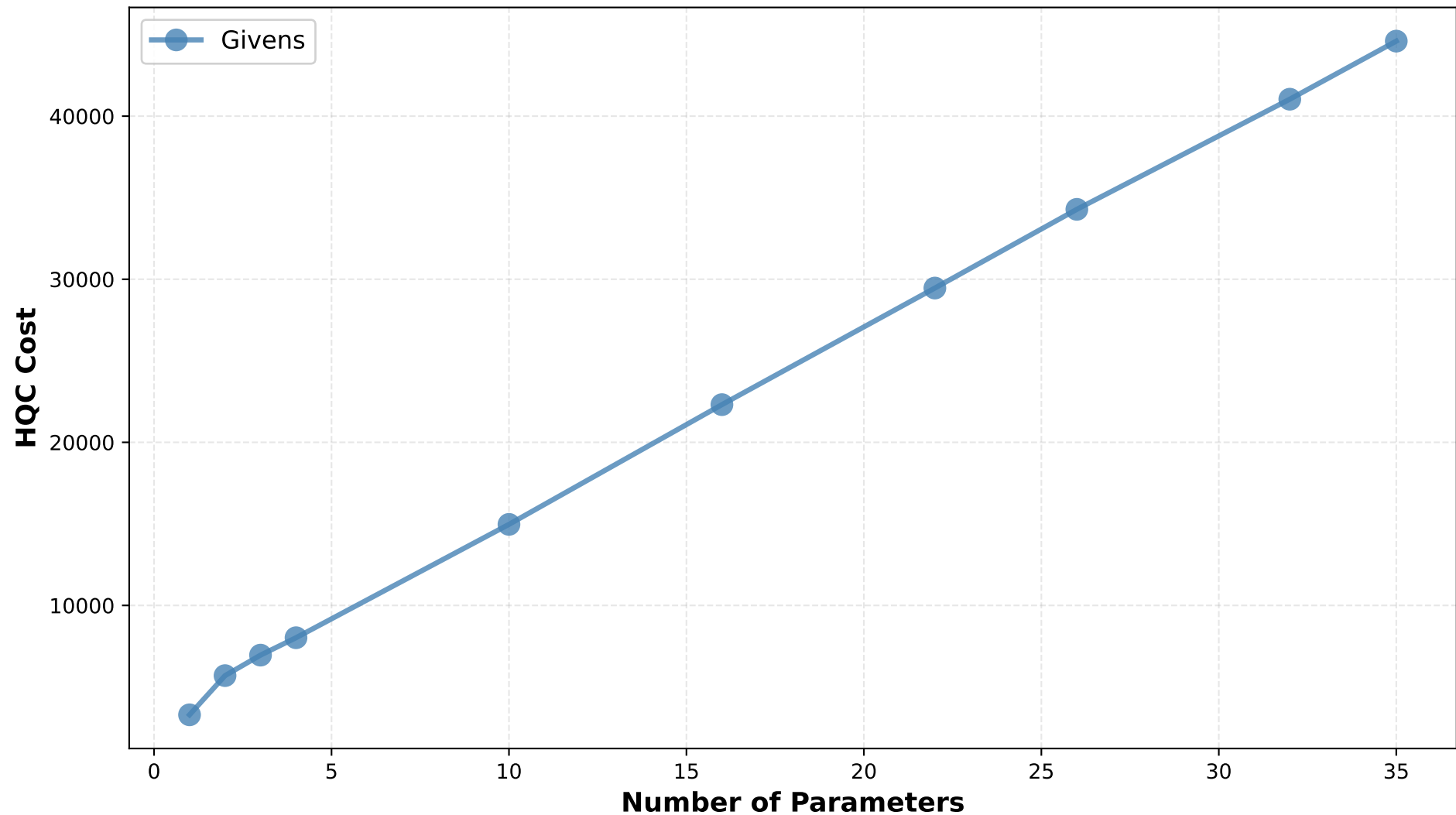
N2 - HQC Cost vs Number of Parameters (H1-1E)
