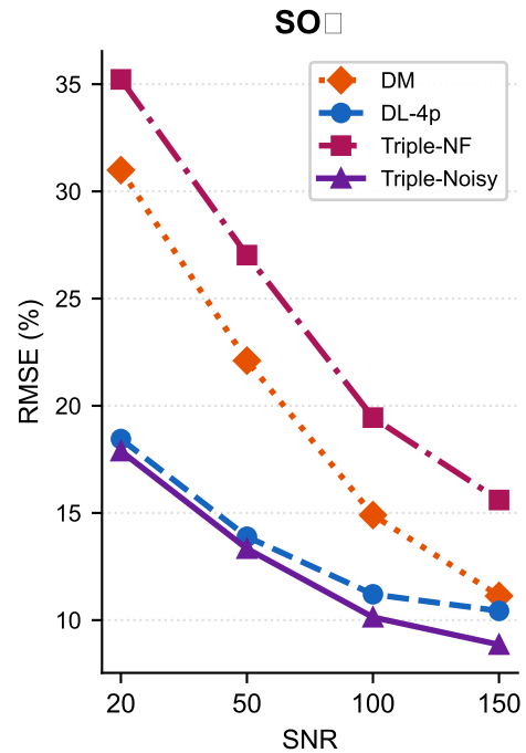
Ablation: RMSE vs SNR — DM vs DL-4p vs Triple-NF vs Triple-Noisy
