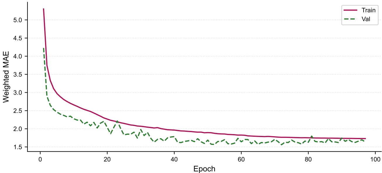
Triple-Regime NF (A+B+C) — Training Curve
