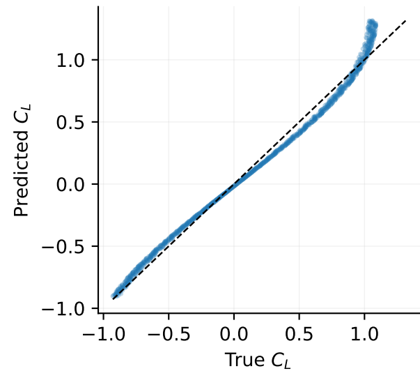
Sparse RMSE=0.0042
