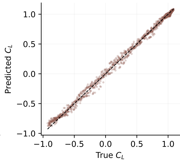
RBF RMSE=0.0440
