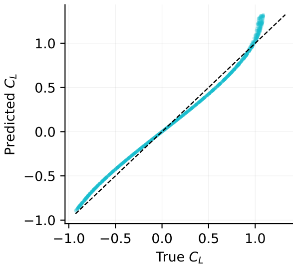
Physics RMSE=0.0759
