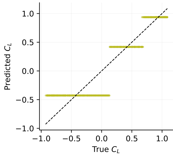
Rule/tree RMSE=0.2297
