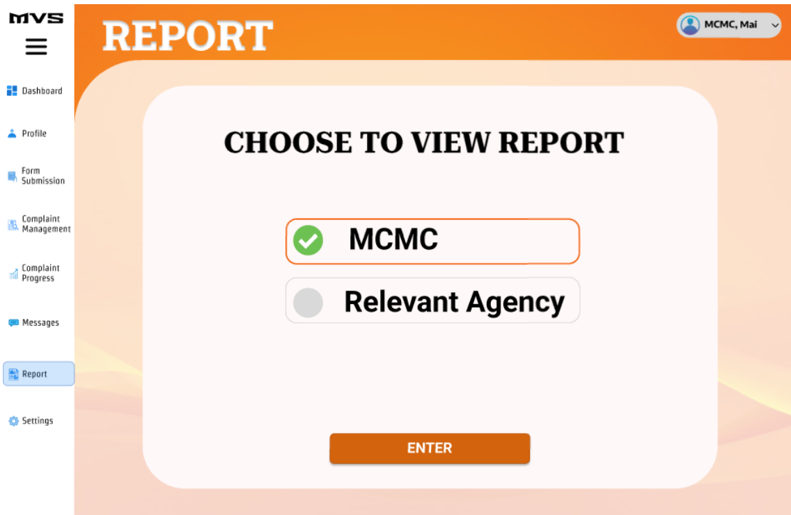
Figure 3.27 MCMC Report
