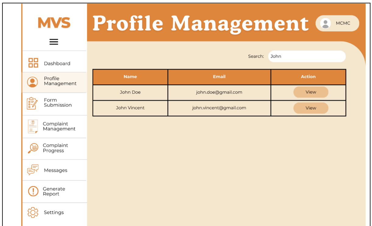
Figure 3.22 MCMC Search
