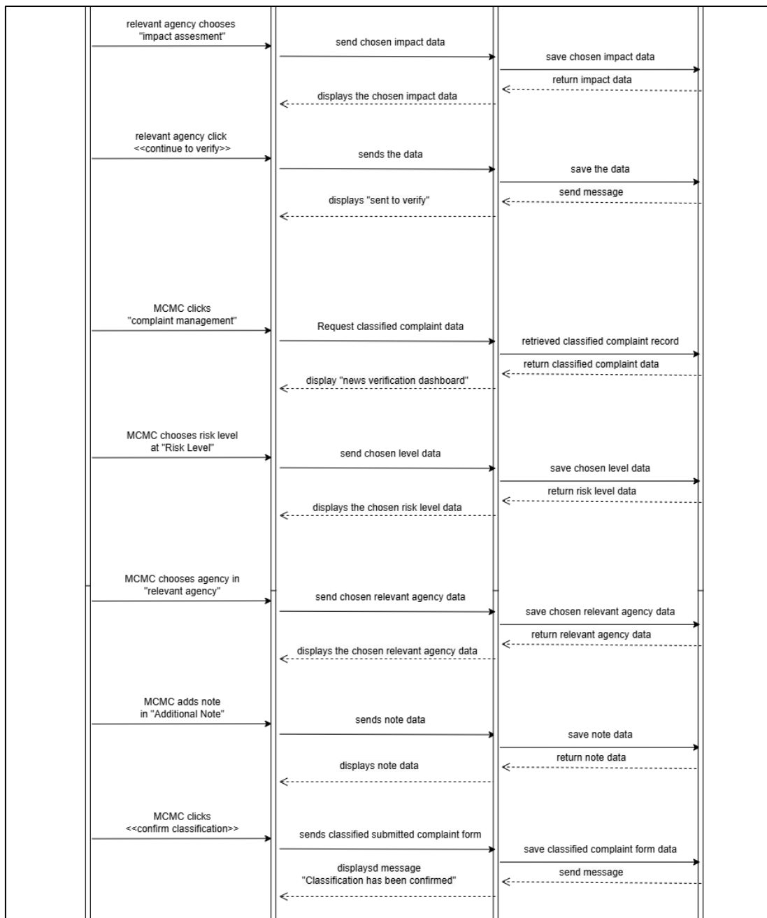
Figure 3.43 Basic Flow for Manage Assigned Complaint Form
