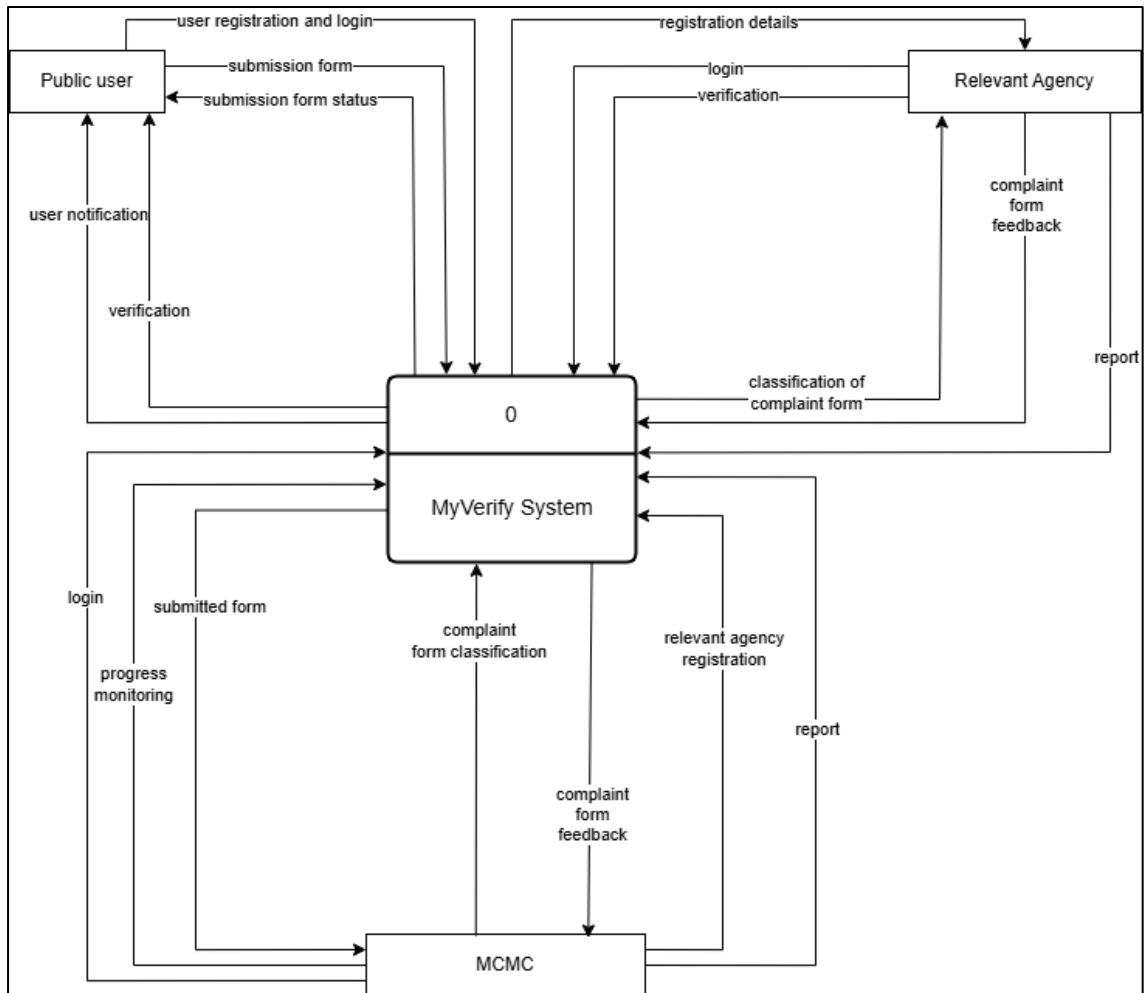
Figure 2.1 Context Diagram
