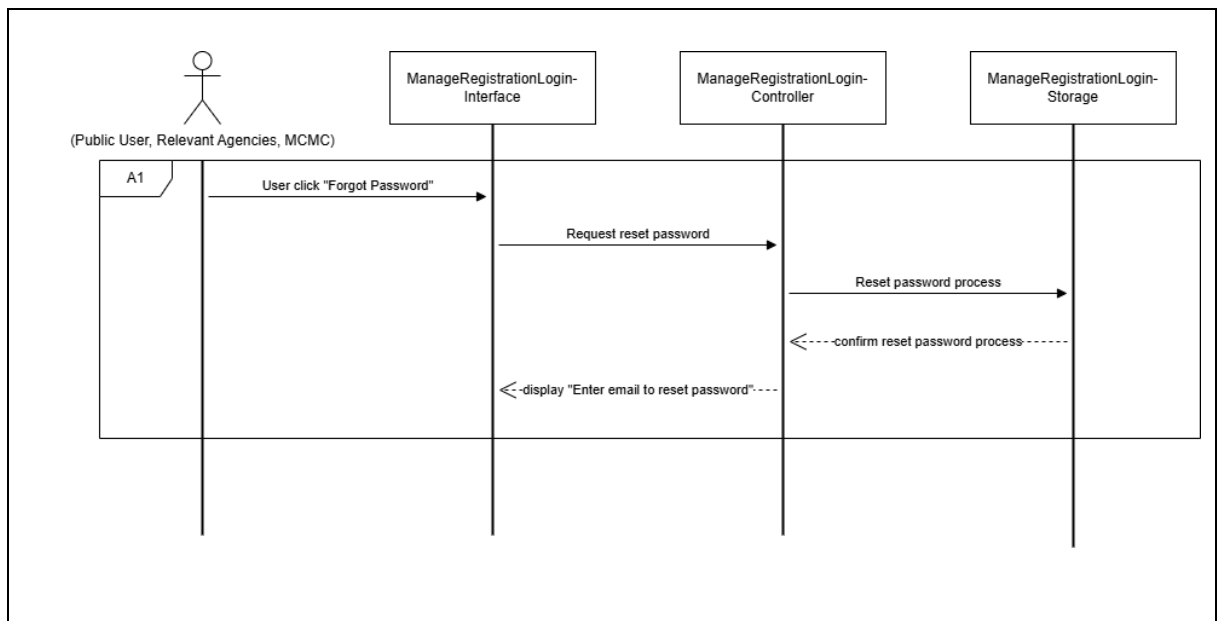
Figure 3.3 Alternative Flow for Registration & Login
