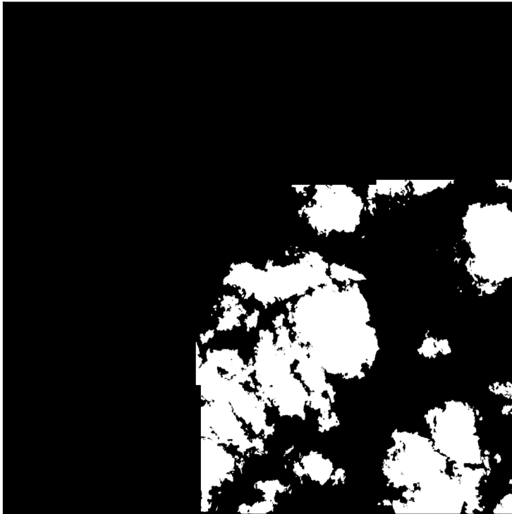
Ground truth
