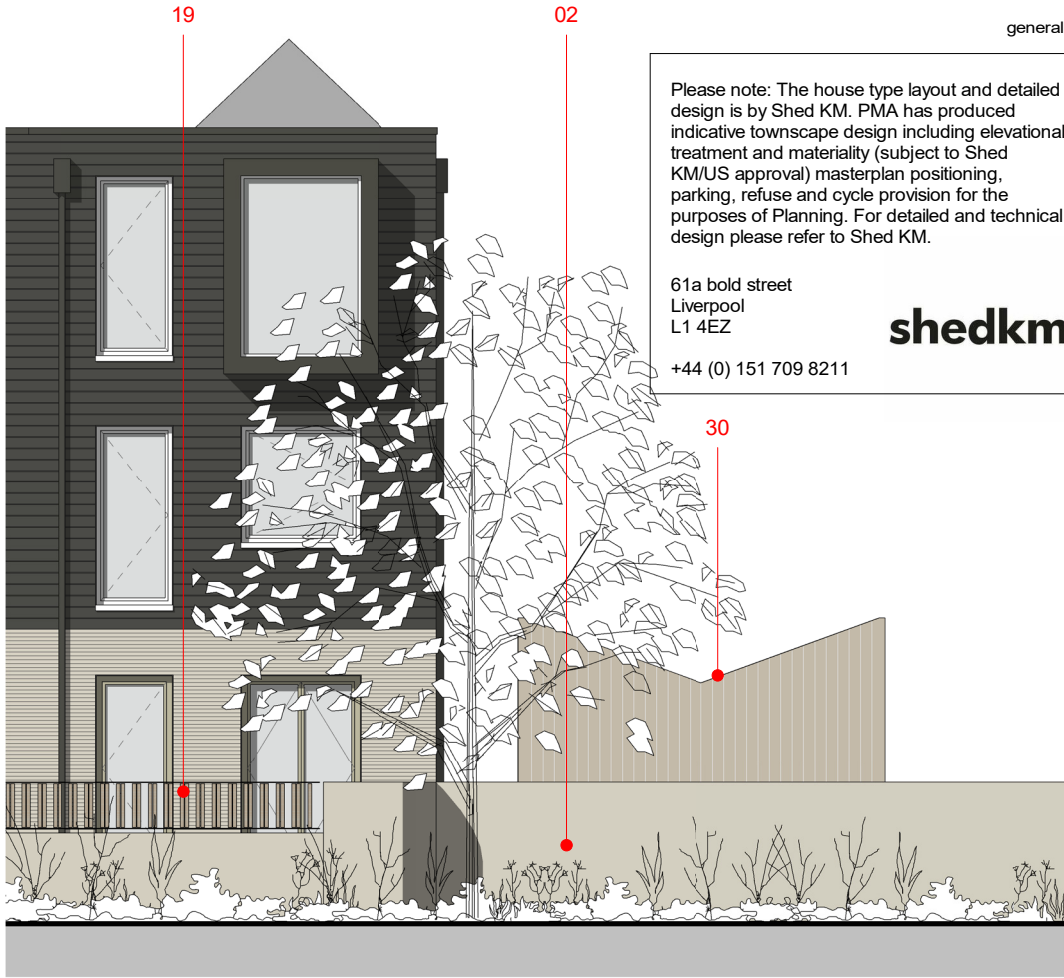
Rear (from landscape) Elevation - 1:100
