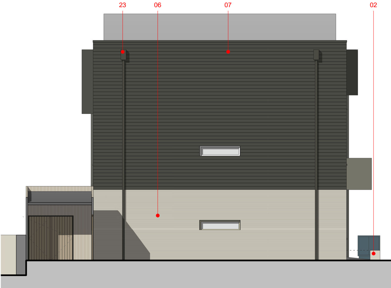
Side Elevation - Kitchen Side Standard Gable - 1:100
