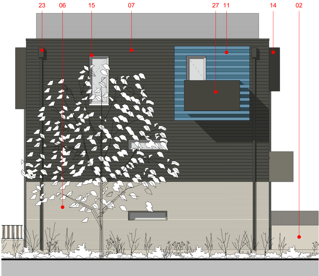
Side Elevation - Kitchen Side Special Gable - 1:100
