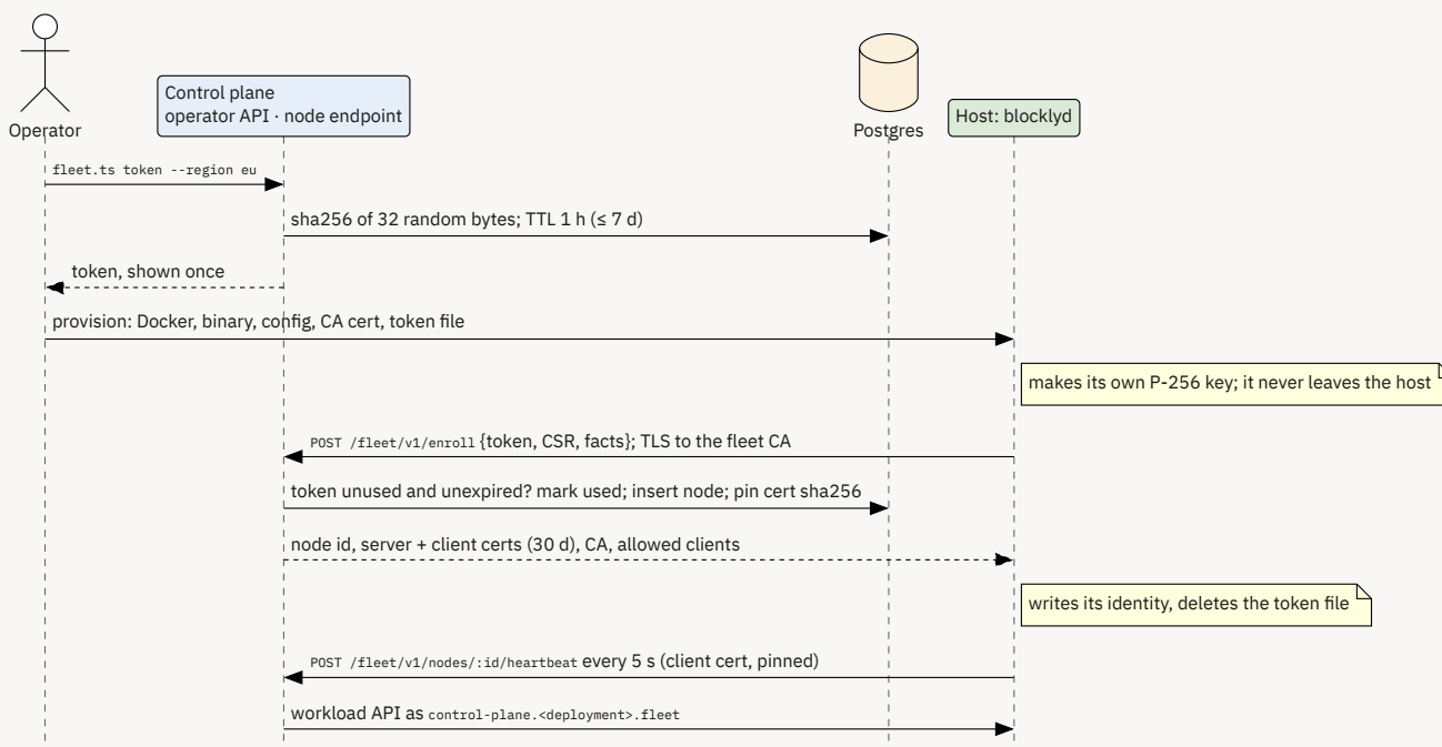
Figure 11: Enrollment. apps/control/src/infra/fleet/node-endpoint.ts:17, apps/control/src/infra/fleet/registry.ts:168, apps/blocklyd/src/fleet/enroll.rs:30.
