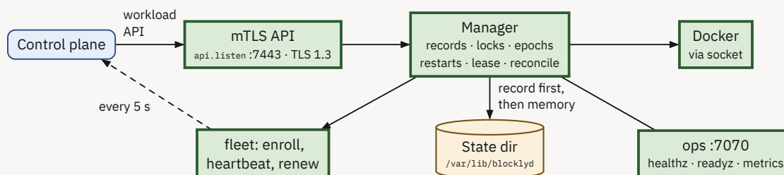
Figure 7: blocklyd's parts. apps/blocklyd/src/manager.rs (3,296 lines) is the core; apps/blocklyd/src/api/mod.rs:460 the routes; apps/blocklyd/src/fleet/heartbeat.rs.
