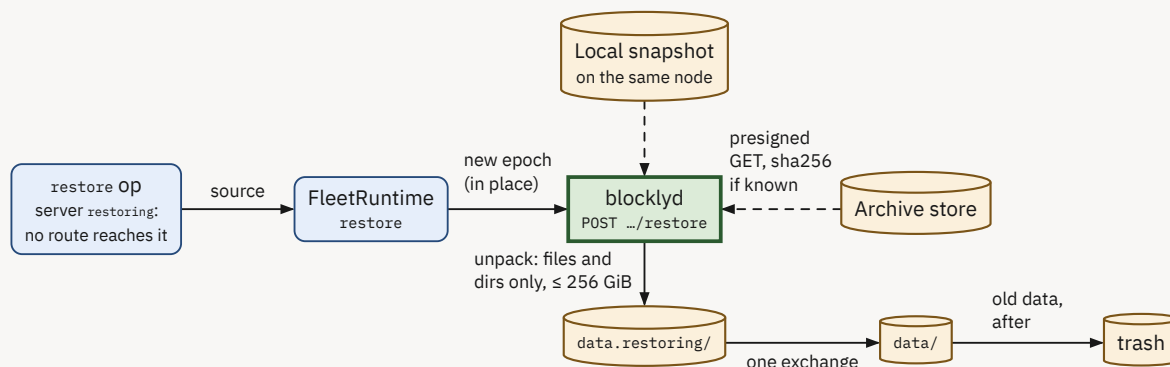
Figure 20: A restore. The new data is assembled beside the old, so a bad archive costs nothing. apps/blocklyd/src/manager.rs:1426 , apps/blocklyd/src/transfer.rs:161 , apps/control/src/infra/fleet/fleet-runtime.ts:980 .
