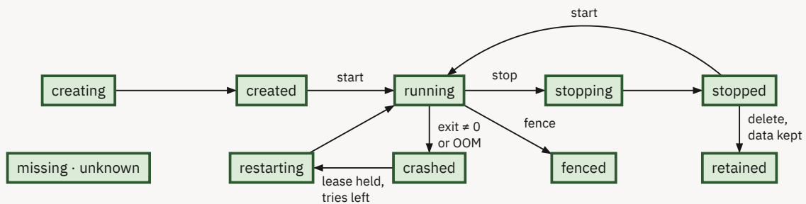
Figure 16: A workload on a node (WorkloadState, apps/blocklyd/src/protocol.rs:495), derived from blocklyd's record and Docker's view (apps/blocklyd/src/manager.rs:3217). A superseded copy at rest reads fenced ; a stopped or crashed copy waiting to resume after a reboot reads restarting ; missing : the container vanished; unknown : Docker doesn't answer.
