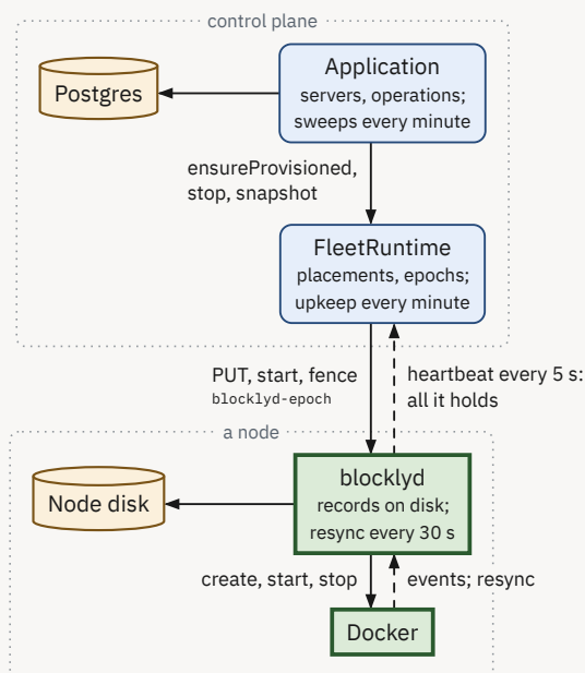
Figure 10: Three owners, three loops; FleetRuntime keeps its tables in the same Postgres. Solid: calls; dashed: reports. Sweeps: apps/control/src/infra/pg/jobs.ts:266 blocklyd intervals: apps/blocklyd/src/config.rs:346.
