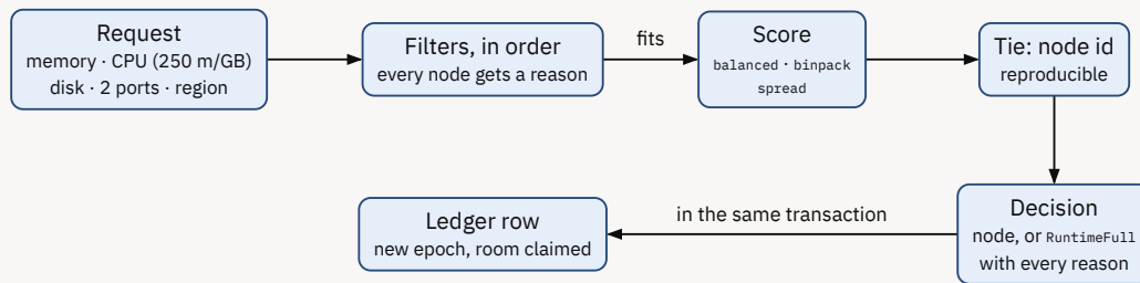
Figure 9: Placement. A refusal reads like memory: 900 MB free after headroom, needs 3072 .
