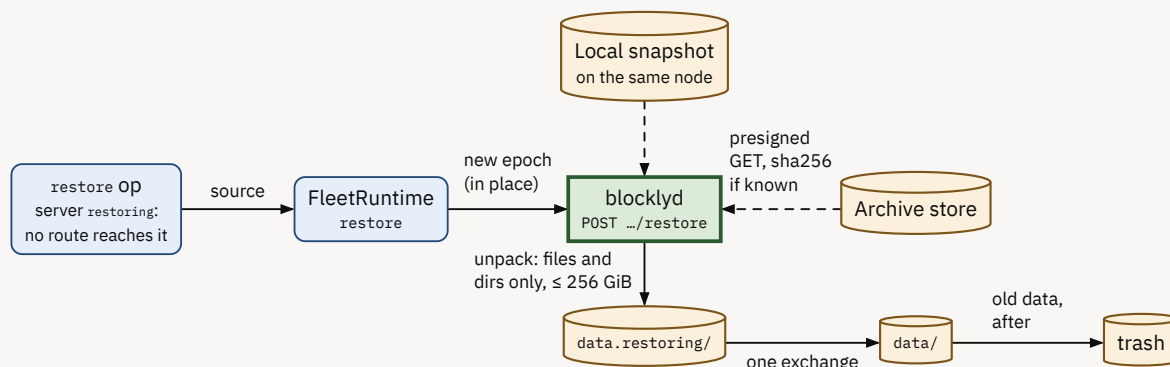
Figure 20: A restore. The new data is assembled beside the old, so a bad archive costs nothing. blocklyd/src/manager.rs:1426 , blocklyd/src/transfer.rs:161 , apps/control/src/infra/fleet/fleet-runtime.ts:980 .
