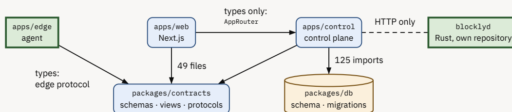
Figure 3: Package dependencies. packages/contracts depends only on zod ; packages/db only on drizzle-orm and pg . blocklyd shares no code with the TypeScript packages: it and the control plane speak HTTP.
