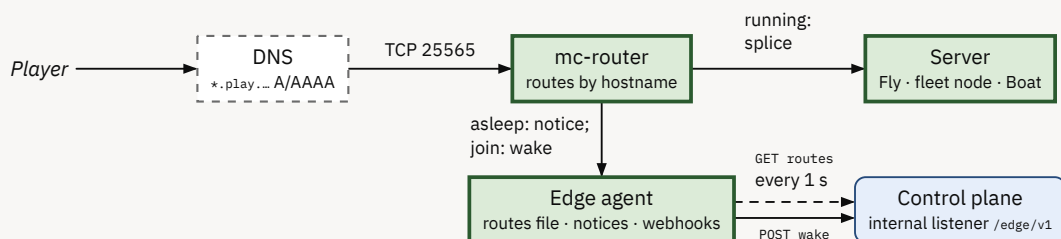
Figure 25: The player's path. Routes are pulled, never pushed: every edge converges and a restart loses nothing. apps/edge/agent.ts:44 .
