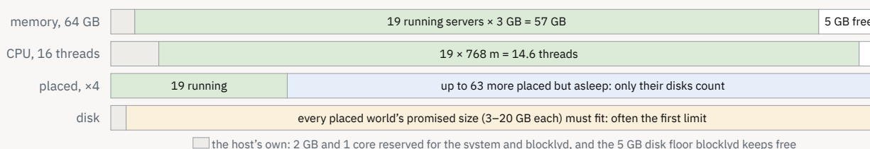
Figure 8: A 64 GB, 8-core/16-thread node (an OVH RISE-S) with 3 GB servers, at the defaults: host reserve 2 GB and 1 core (blocklyd), 250 m of CPU per GB, placed memory \leq 4 \times allocatable. Memory alone fits 20 running; the CPU ledger stops at 19. apps/control/src/infra/fleet/placement.test.ts:191 checks the same arithmetic: 19 running, 78 asleep on a 60,000 MB node.
