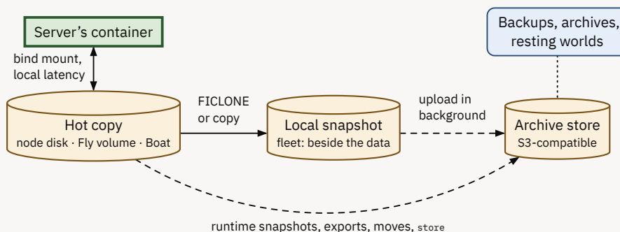
Figure 18: Hot and durable copies. The local snapshot tier exists only on the fleet; other runtimes snapshot with their provider (§27).
