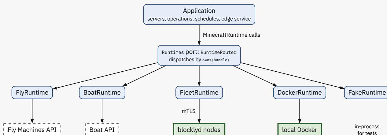
Figure 4: One port, five adapters. The router is in the path even with one runtime. apps/control/src/app/runtimes/router.ts:131 , apps/control/src/main.node.ts:105 .
