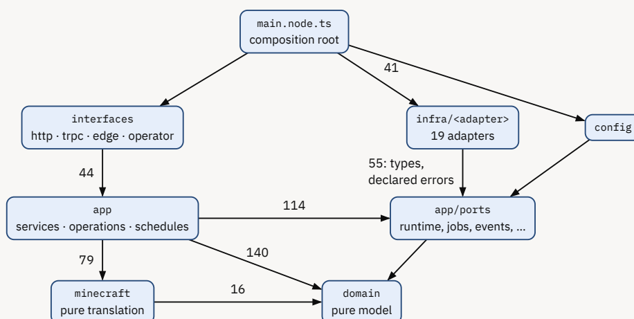
Figure 2: Control-plane layers and measured import counts (production files). No adapter imports another adapter; only main imports adapters. scripts/check-boundaries.ts:133 .
