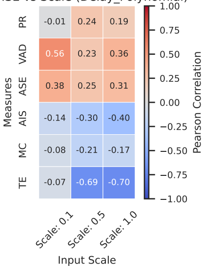
NMSE vs Scale (Delay_Polynomial)
