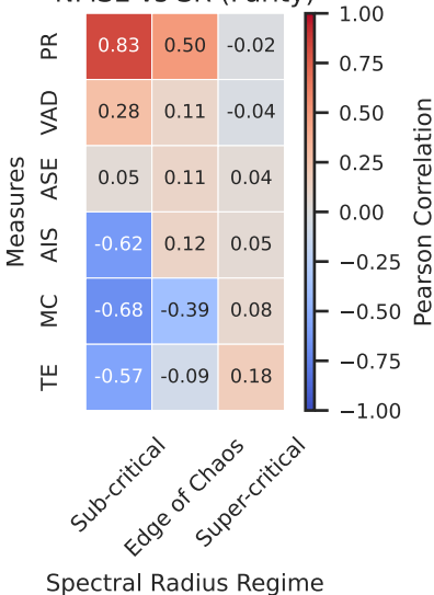
NMSE vs SR (Parity)
