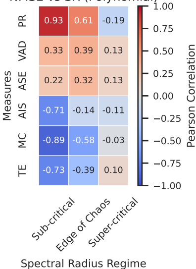
NMSE vs SR (Polynomial)
