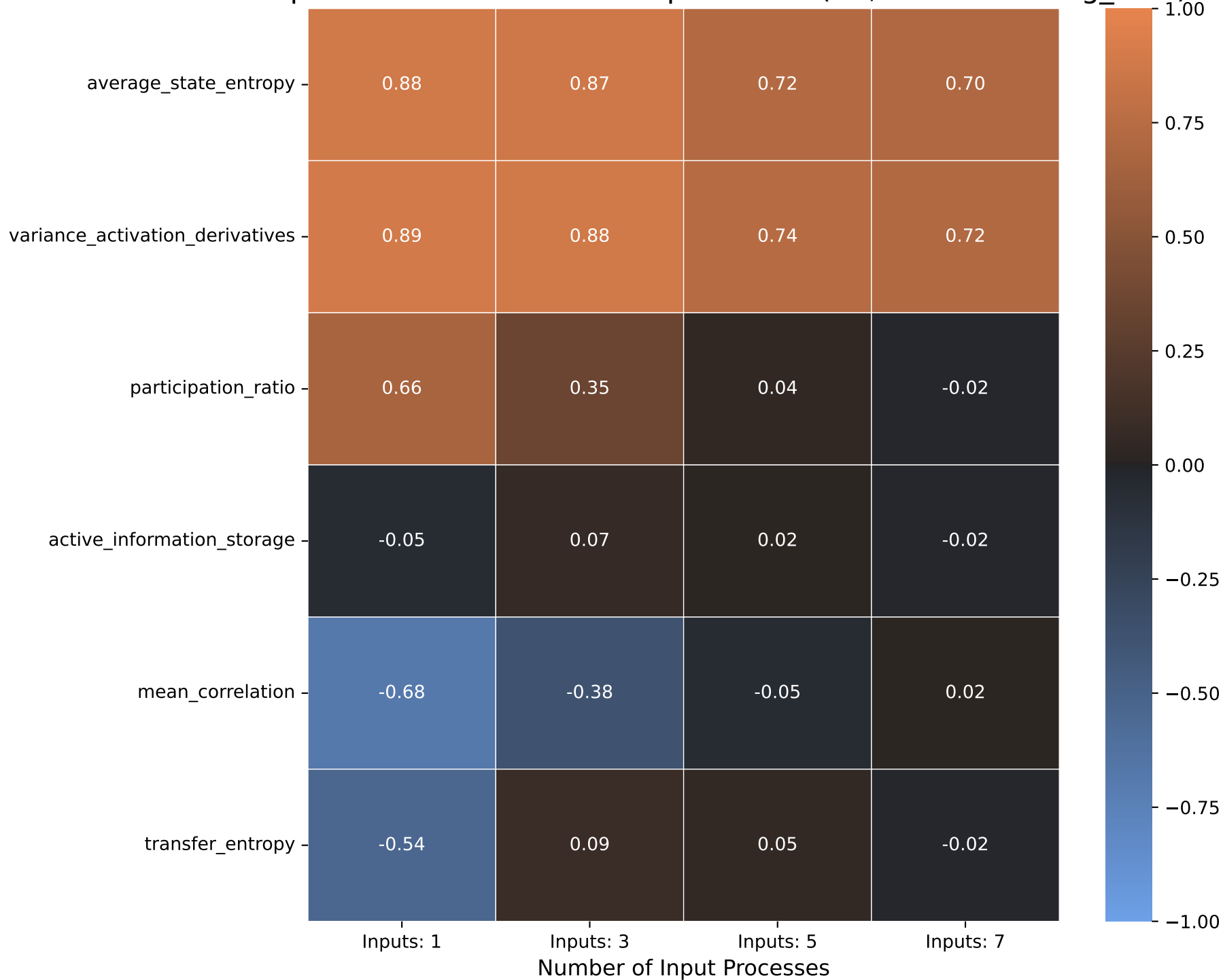
NMSE Spearman Correlation vs Input Count (RP, Task: Counting_Task)
