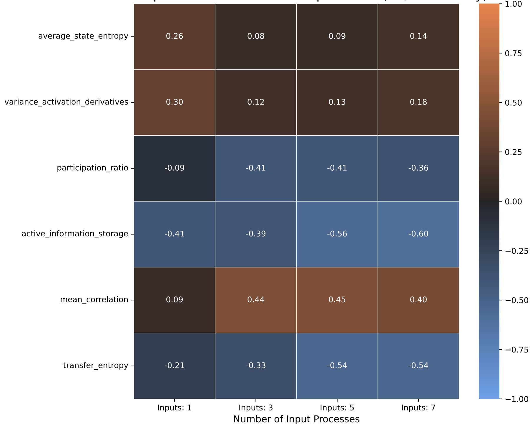
NMSE Spearman Correlation vs Input Count (RP, Task: Delay)
