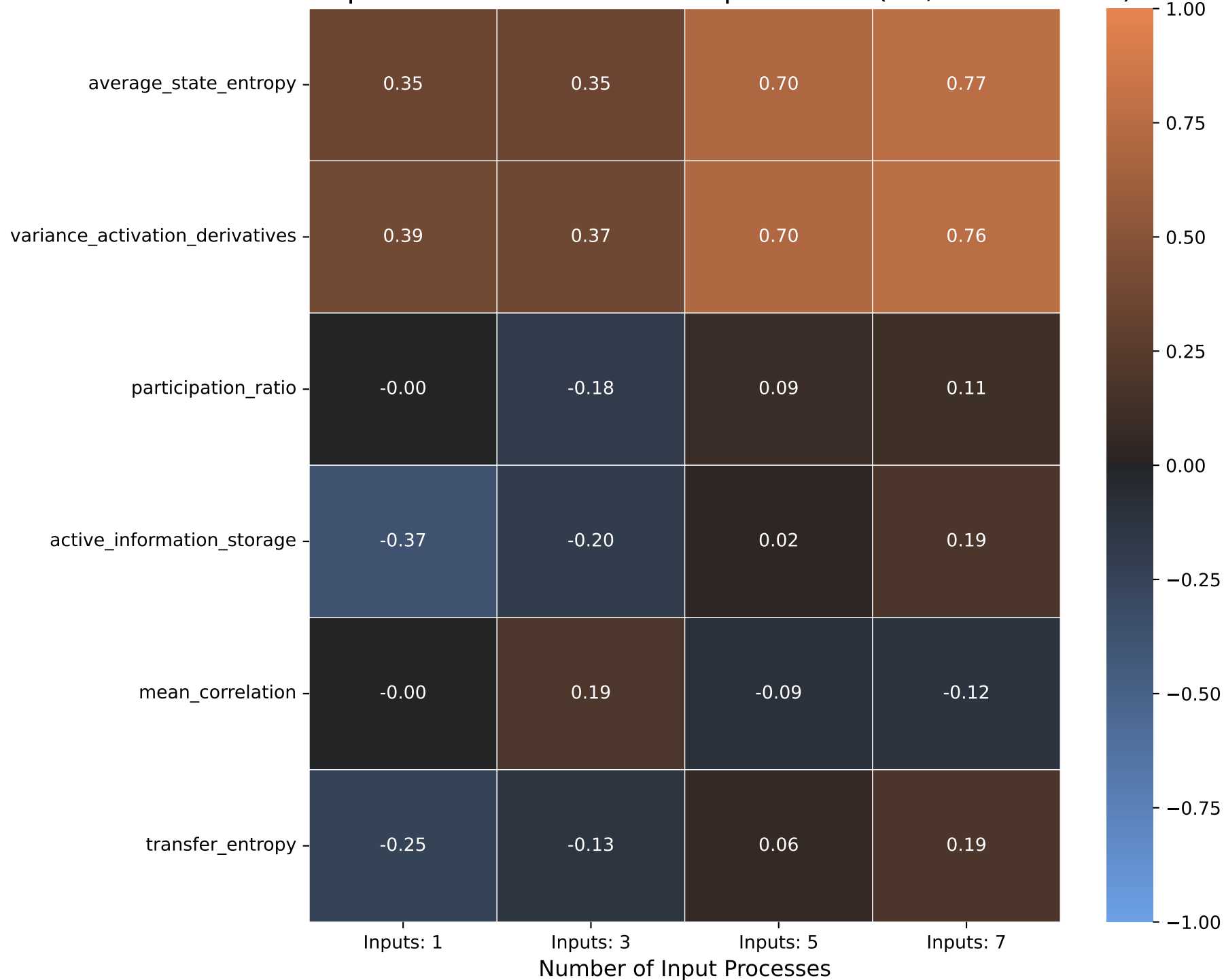
NMSE Spearman Correlation vs Input Count (RP, Task: Narma)
