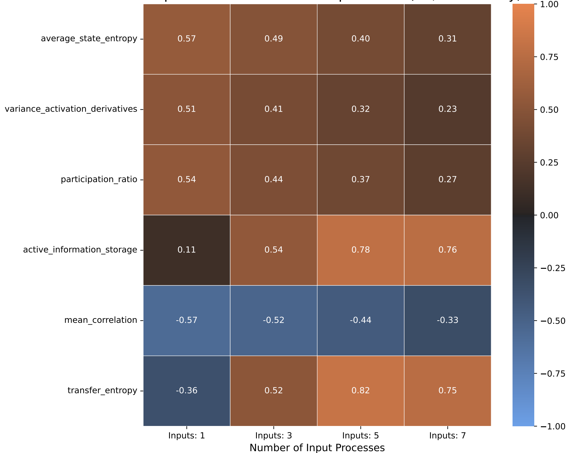
NMSE Spearman Correlation vs Input Count (RP, Task: Parity)
