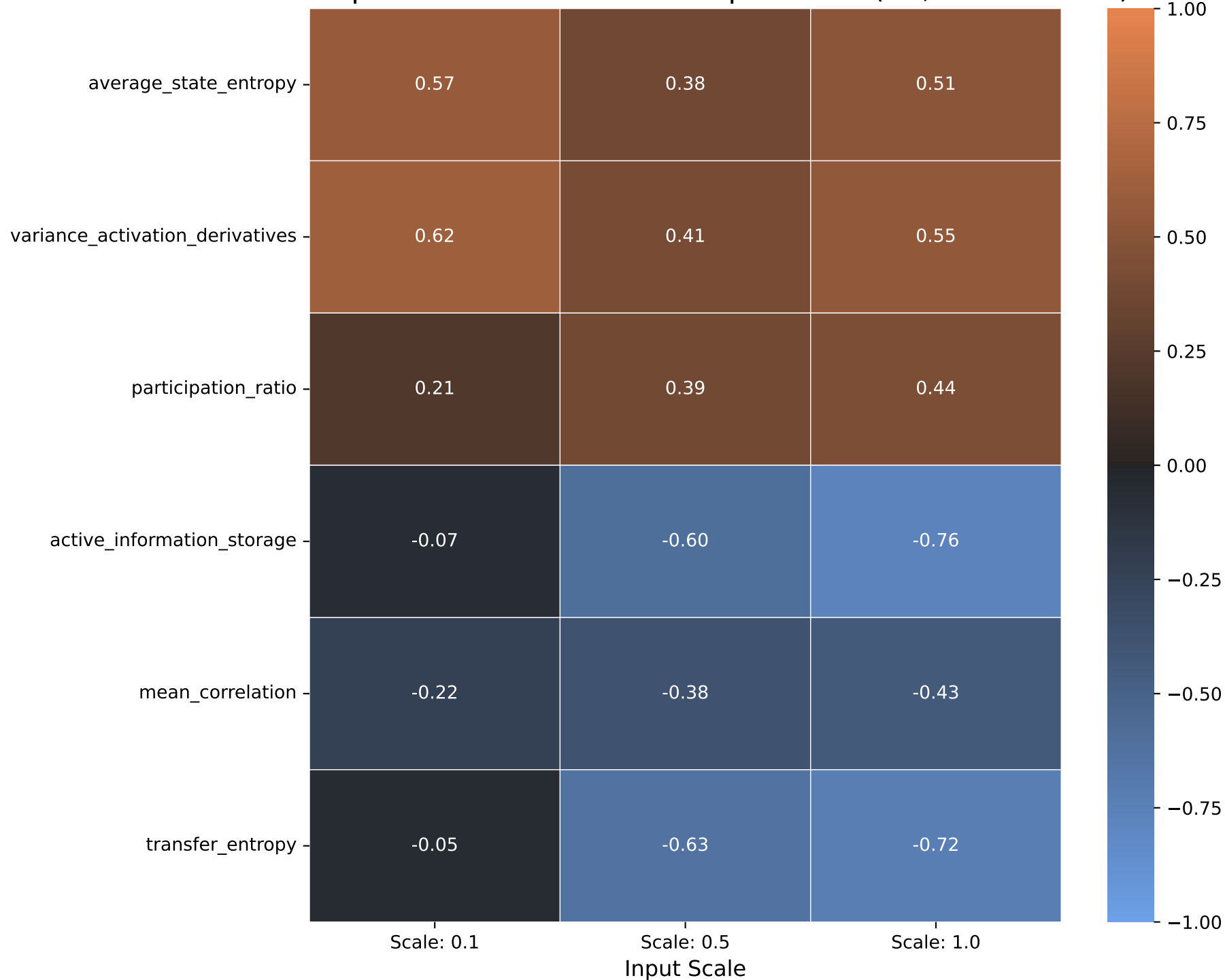
NMSE Spearman Correlation vs Input Scale (RP, Task: Narma)
