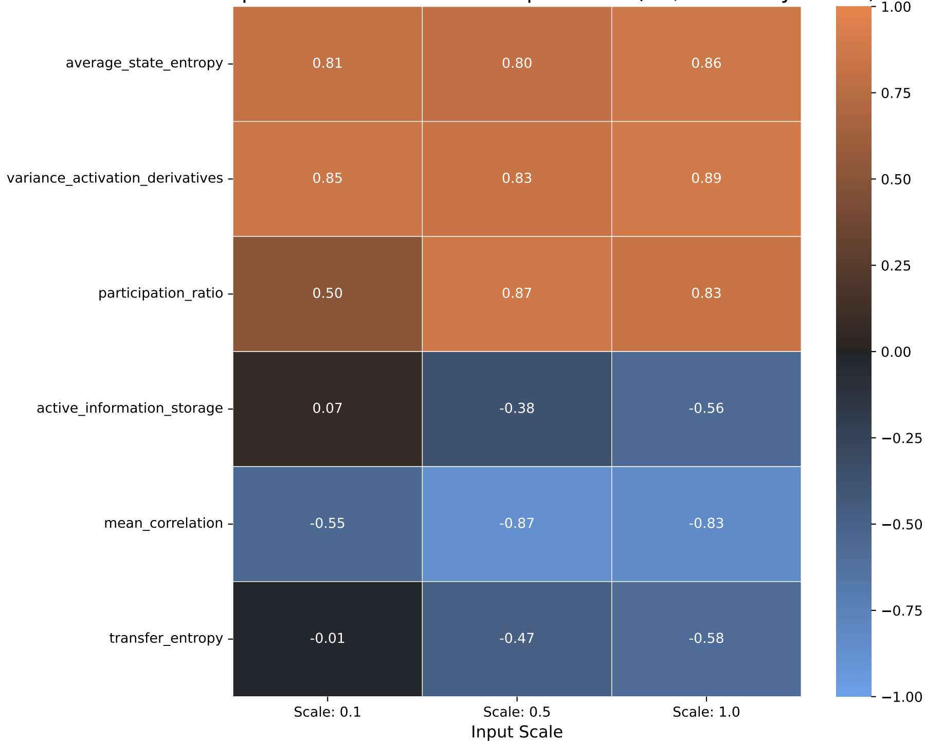
NMSE Spearman Correlation vs Input Scale (RP, Task: Polynomial)
