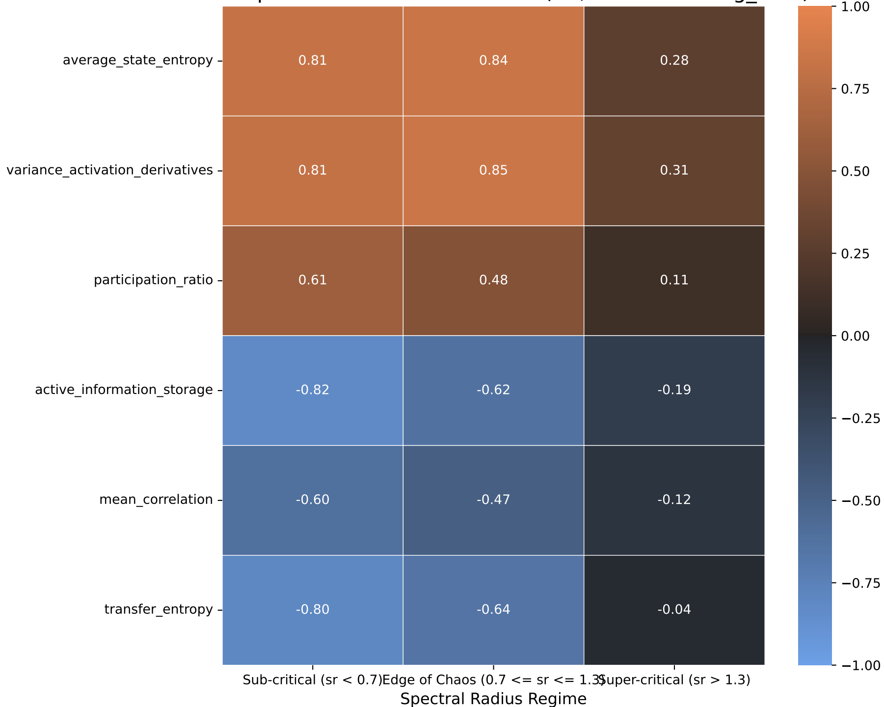
NMSE Spearman Correlation vs SR (RP, Task: Counting_Task)
