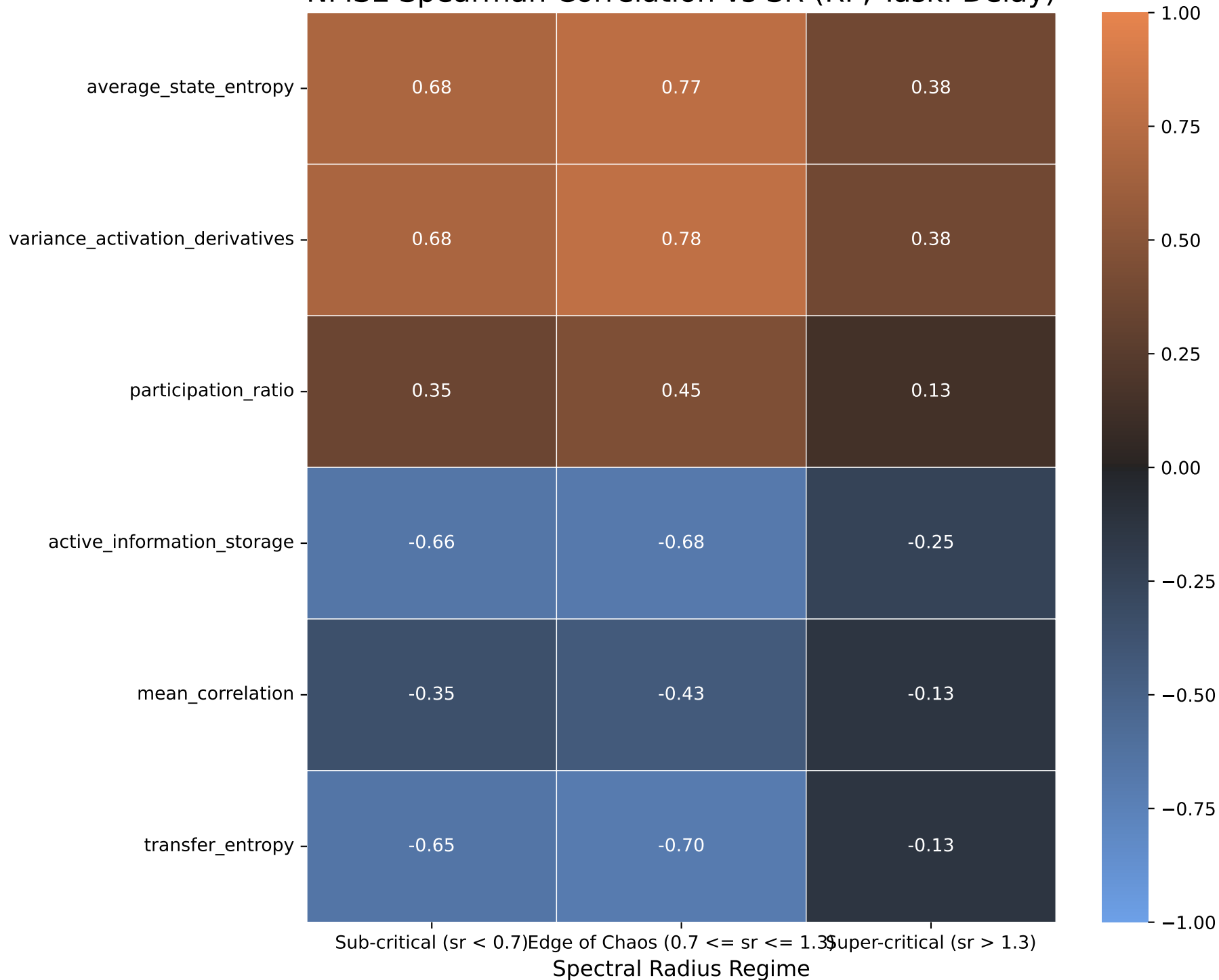
NMSE Spearman Correlation vs SR (RP, Task: Delay)
