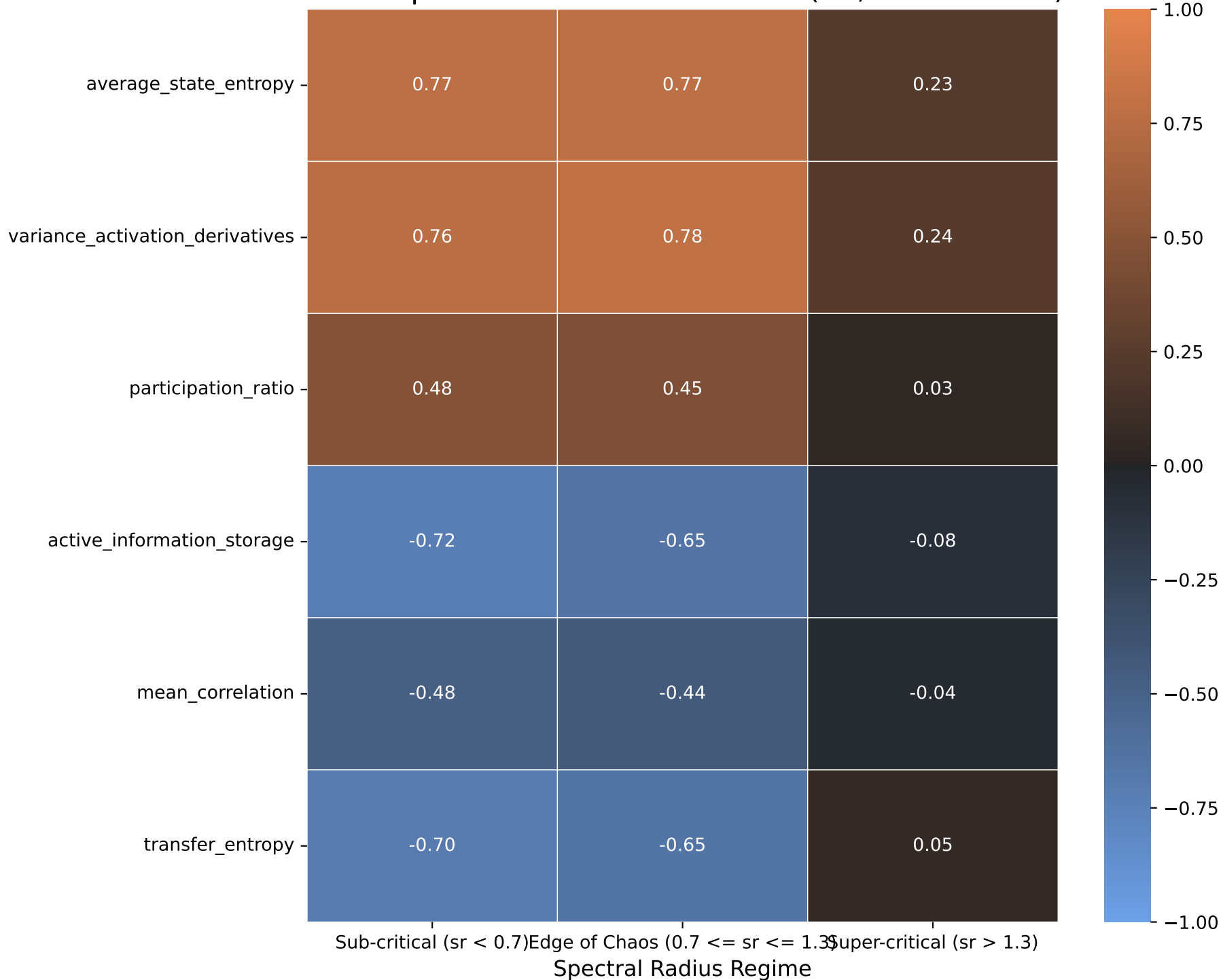
NMSE Spearman Correlation vs SR (RP, Task: Narma)
