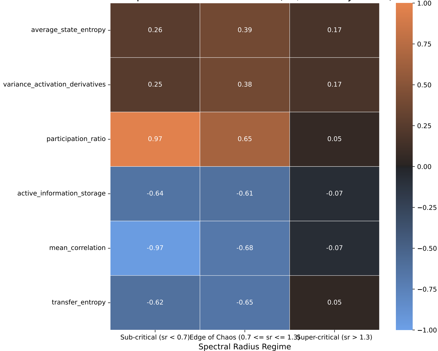
NMSE Spearman Correlation vs SR (RP, Task: Polynomial)
