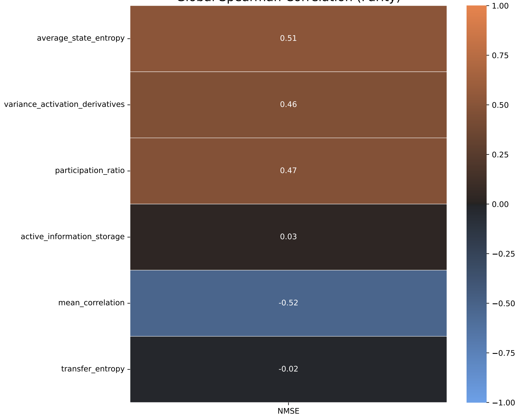
Global Spearman Correlation (Parity)
