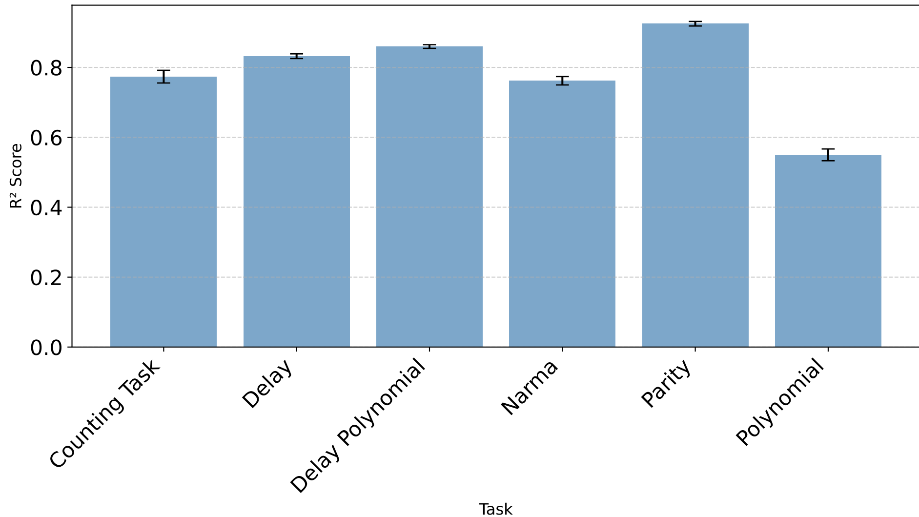
SVR Performance (Test R^2 ) with Standard Deviation
