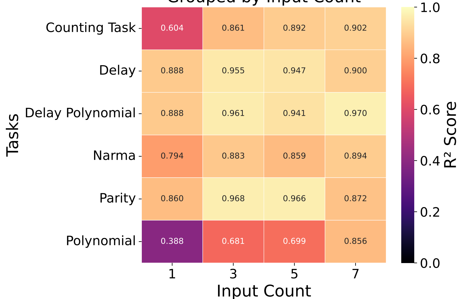
RBF SVR Performance ( R^2 Scores) Grouped by Input Count
