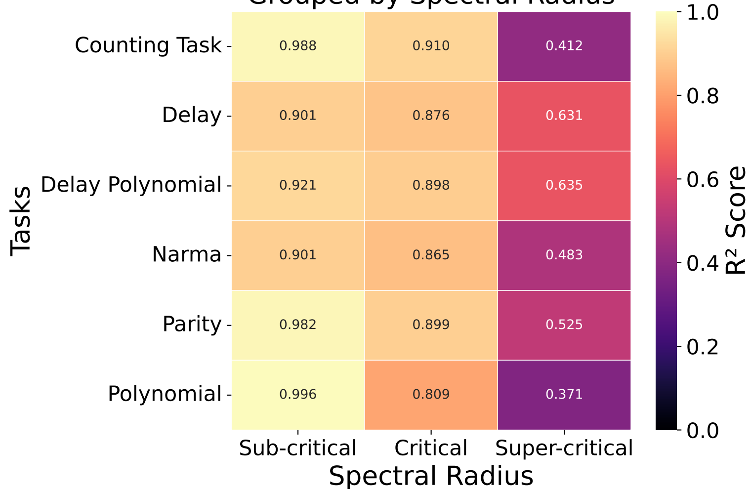
RBF SVR Performance ( R^2 Scores) Grouped by Spectral Radius
