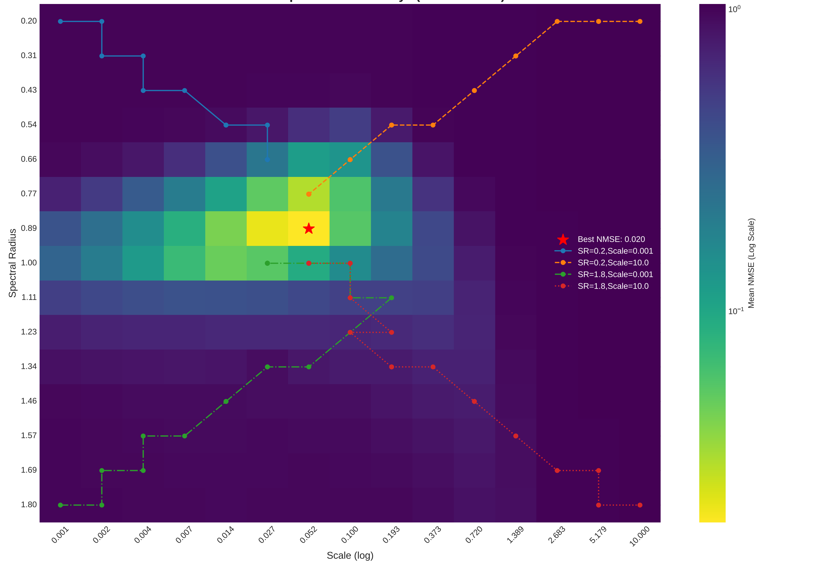
NMSE Landscape for Task: "delay" (Processes: 3)
