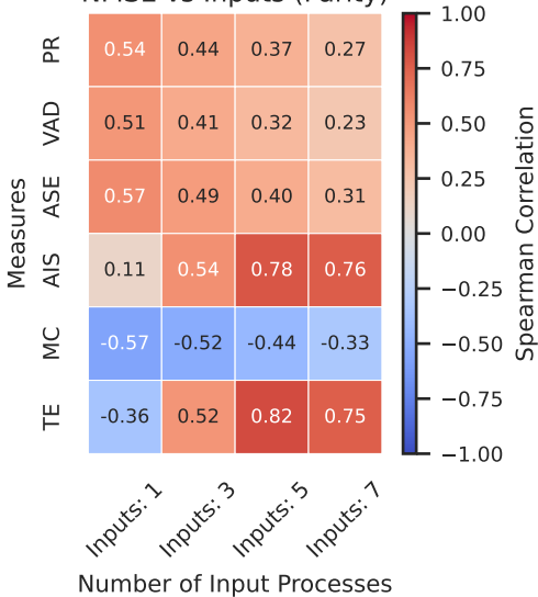
NMSE vs Inputs (Parity)
