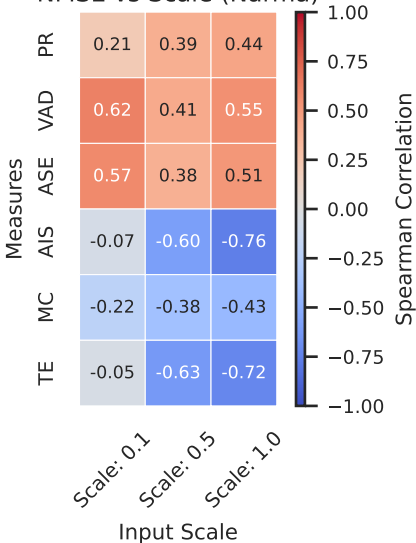
NMSE vs Scale (Narma)
