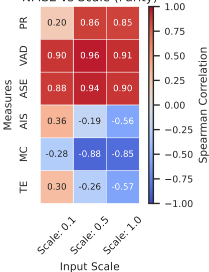
NMSE vs Scale (Parity)
