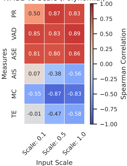
NMSE vs Scale (Polynomial)
