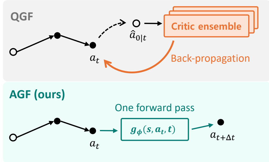
(b) Inference (per flow step)
