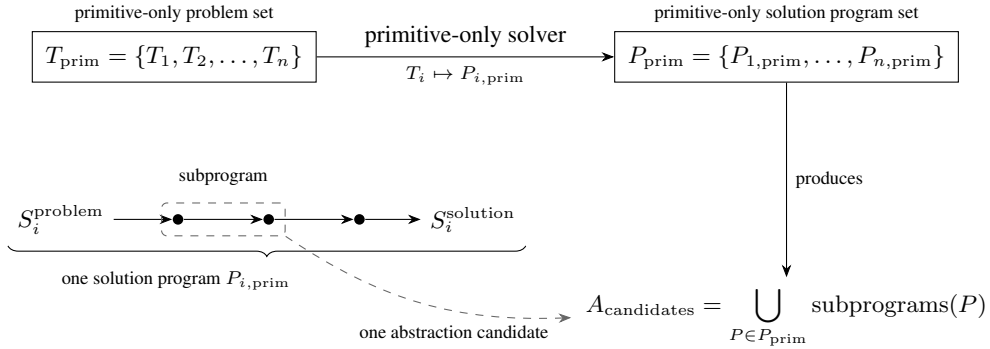
Figure 3: From solver experience to abstraction candidates. The primitive-only solver solves each problem T_i in T_{\text{prim}} , and the solution programs it finds form P_{\text{prim}} , the solver's experience. Every subprogram found within those programs, such as the marked fragment of P_{i,\text{prim}} , enters the abstraction candidate set A_{\text{candidates}} .
