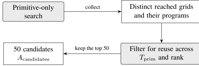
Figure 3: From primitive-only search to abstraction candidates. We first collect the distinct grids reached during search and the programs that produce them. We then check whether each grid could help construct targets across the primitive-only problems, and use this potential for reuse to filter and rank the programs. The top 50 form the candidate set A_{\text{candidates}} shared by both selection procedures.
