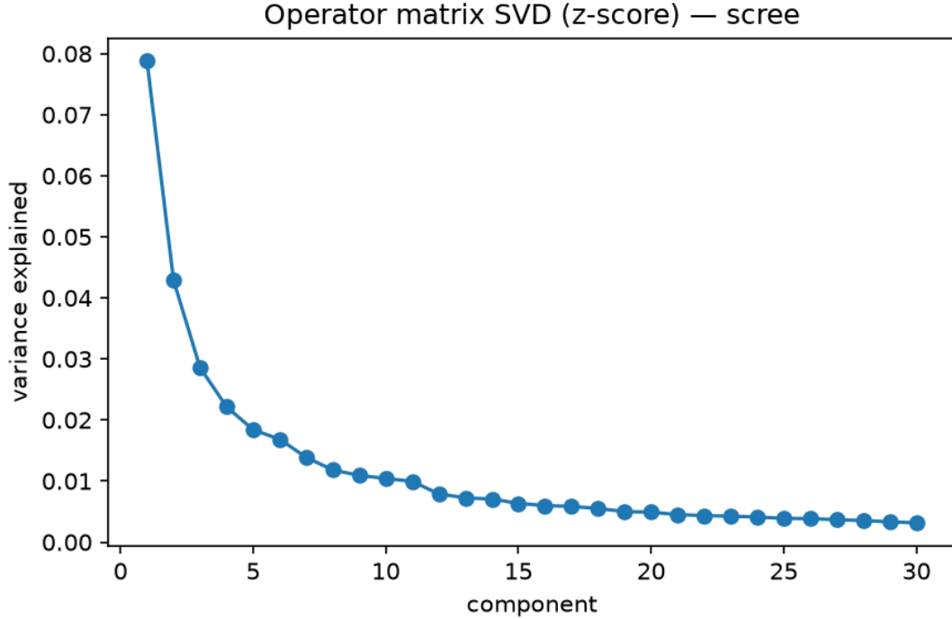
Figure S1. The operator’s own effective rank is far higher than its predictive subspace. Singular-value scree of the 3,106-regulator operator. The spectrum does not collapse after seven components (effective rank \approx 86 ); the \sim 7 -dimensional structure identified in Figure 2 is the transferable part that generalizes to unseen regulators, not the operator’s full rank.
