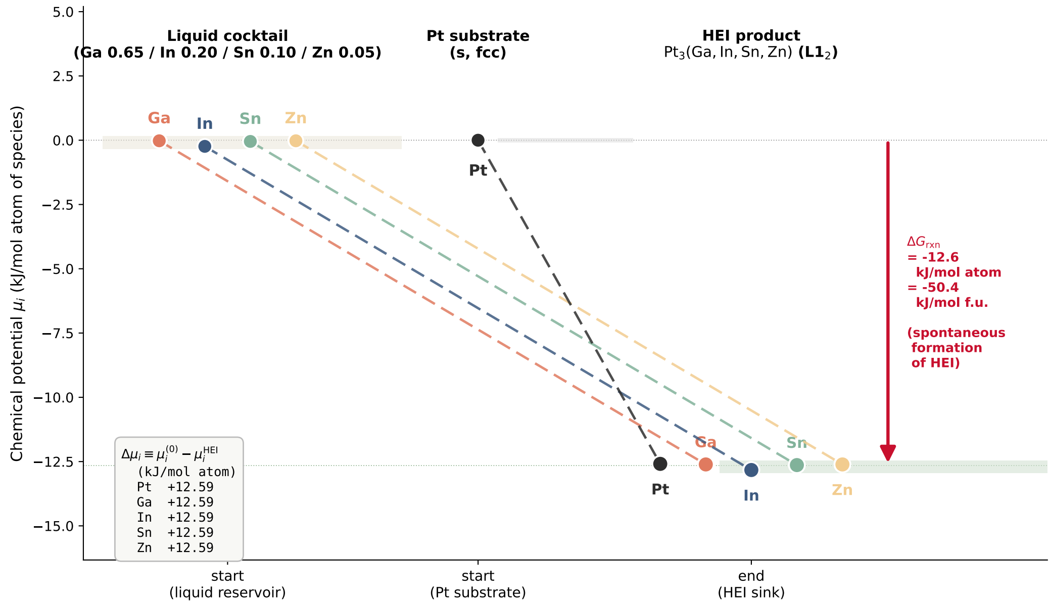
Panel a chemical-potential landscape: liquid reservoir → HEI sink (0 K enthalpic approximation; Ga 0.65 In 0.20 Sn 0.10 Zn 0.05 cocktail)
