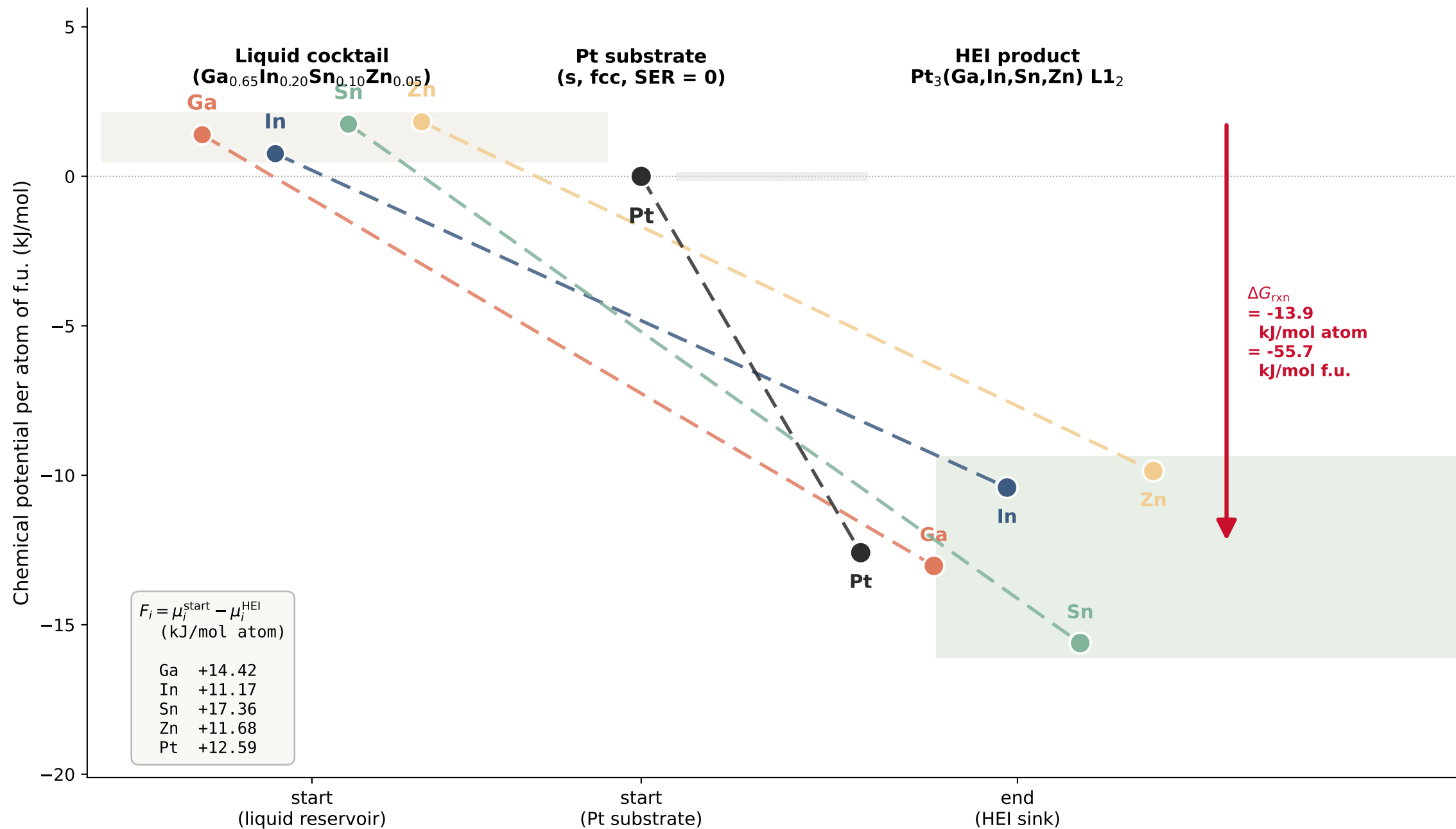
Panel a chemical-potential landscape (SER reference, 0 K enthalpic) liquid reservoir → Pt substrate → HEI sink
