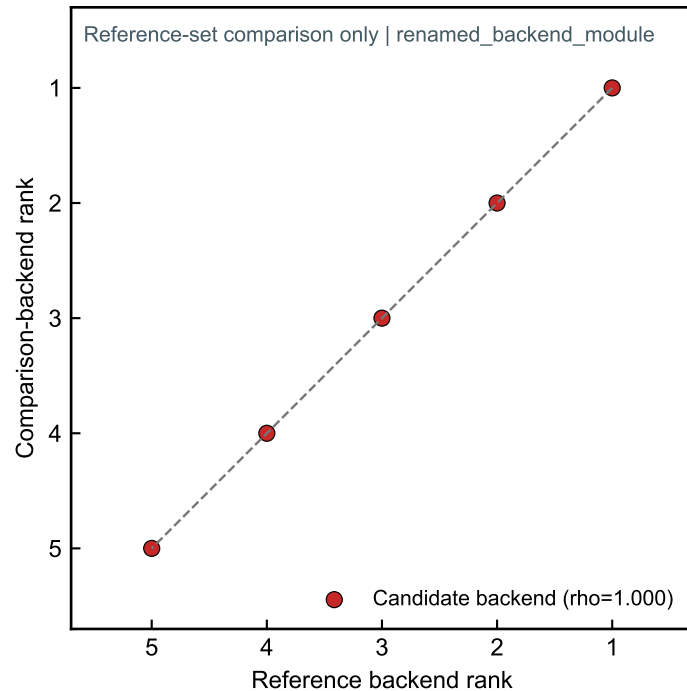
b Reference-set rank consistency
