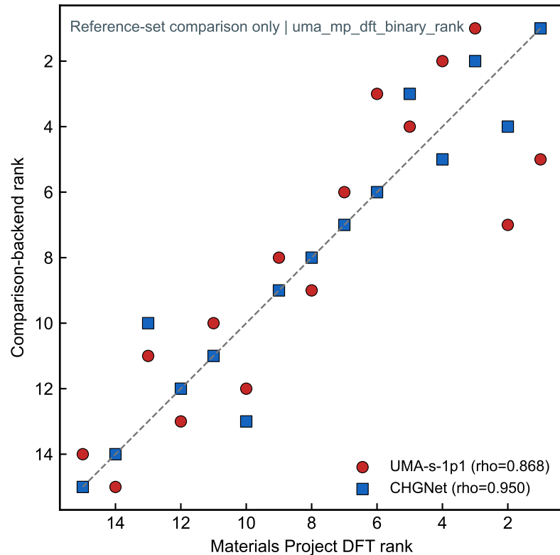
b Reference-set rank consistency
