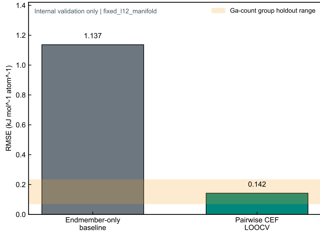
a Fixed-manifold interpolation
