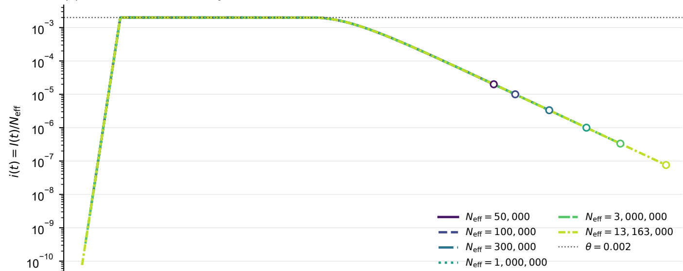
(a) Normalized infection trajectories
