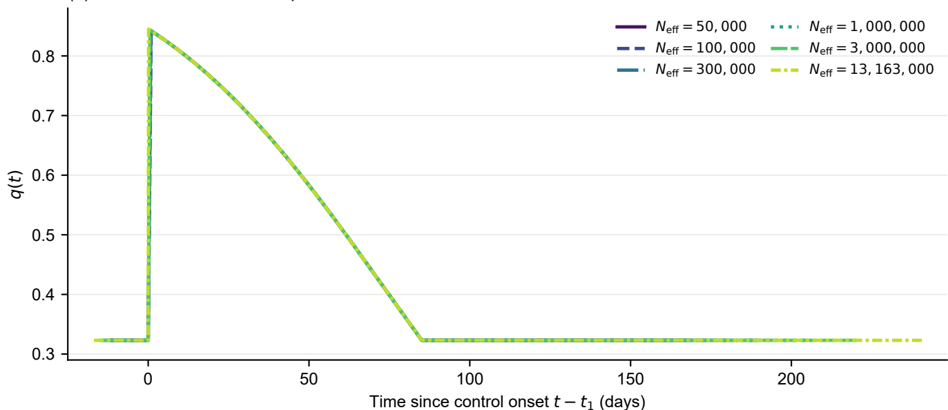
(b) Quarantine-control collapse
