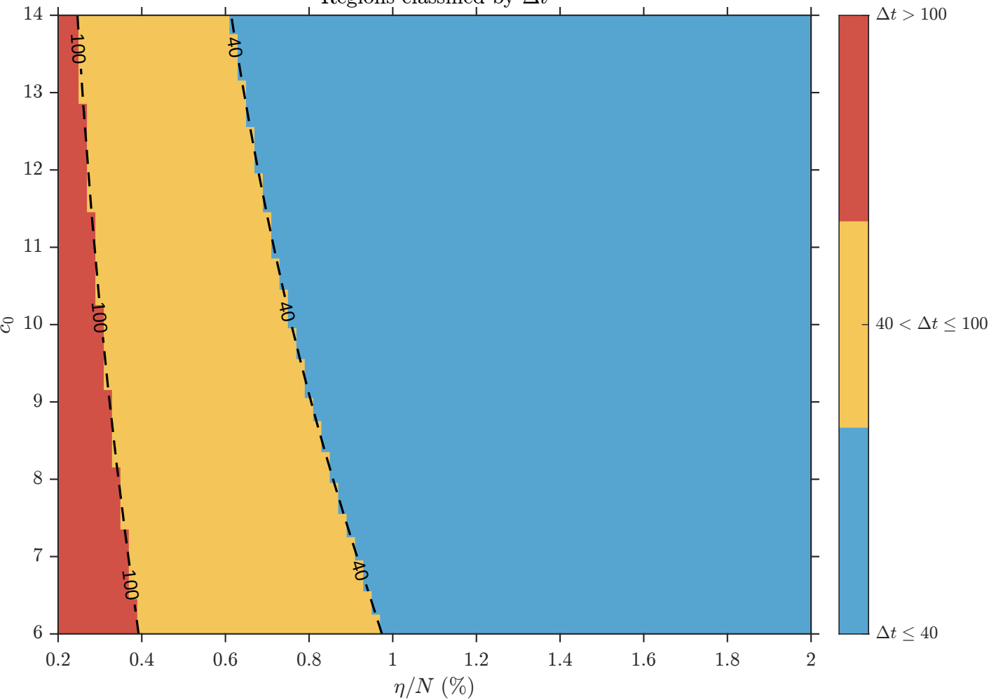
Regions classified by \Delta t
