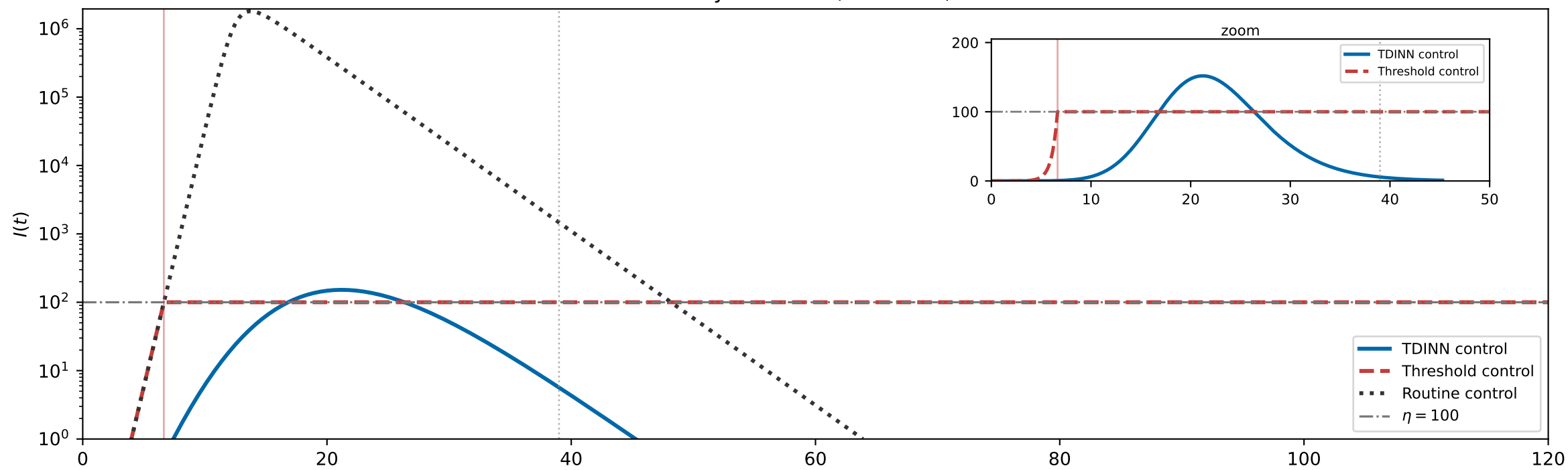
Community infections, \eta=100 , c_0=20
