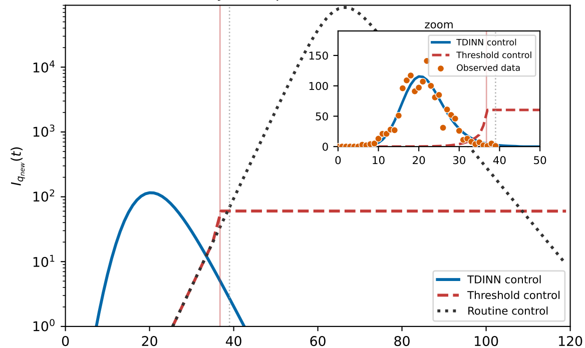
Quarantine rate
