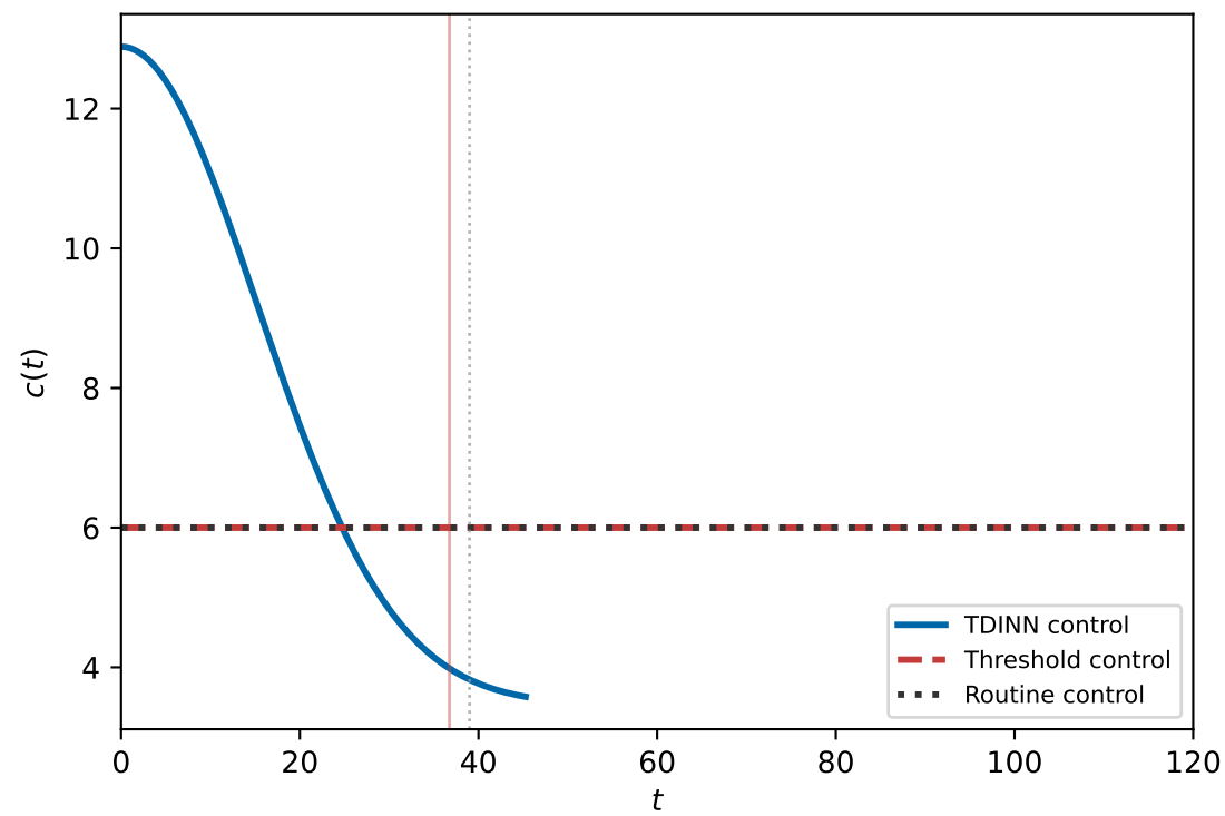
Contact rate
