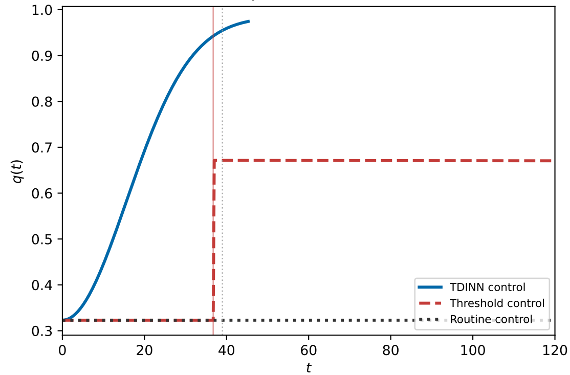
Quarantine rate
