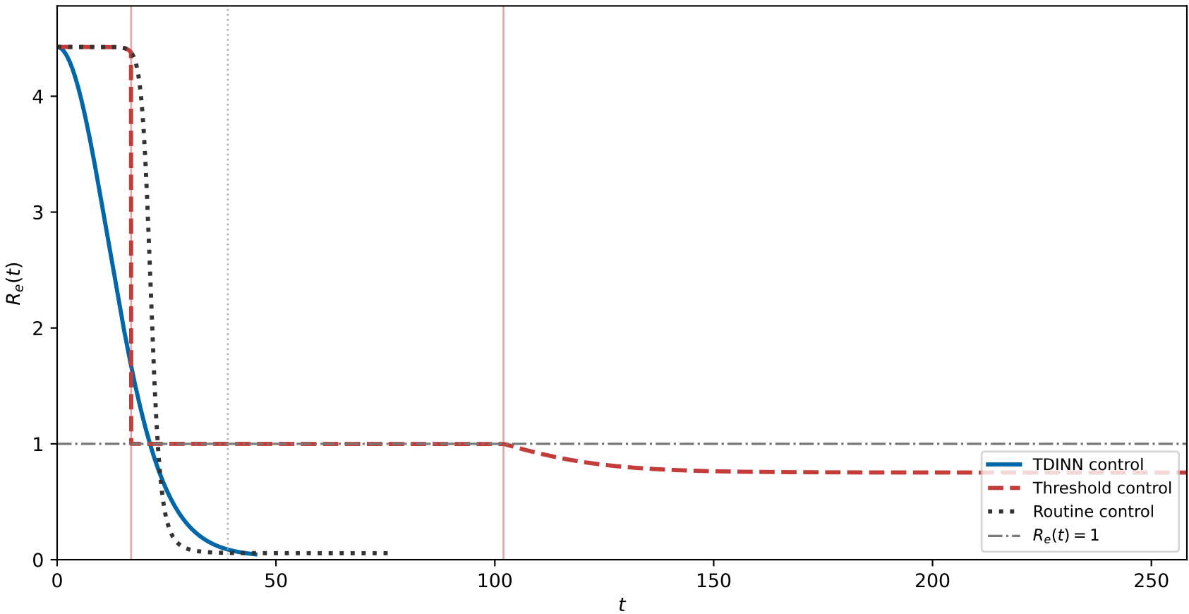
Effective reproduction number
