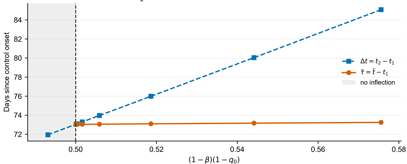
(b) \bar{t} \rightarrow t_2 as (1 - \beta)(1 - q_0) \rightarrow \frac{1}{2}^+
