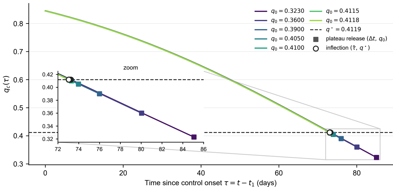
(b) \bar{t} \rightarrow t_2 as (1 - \beta)(1 - q_0) \rightarrow \frac{1}{2}^+
